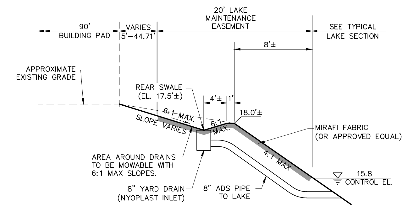
SECTION A-A REAR LOT GRADING NOT TO SCALE
