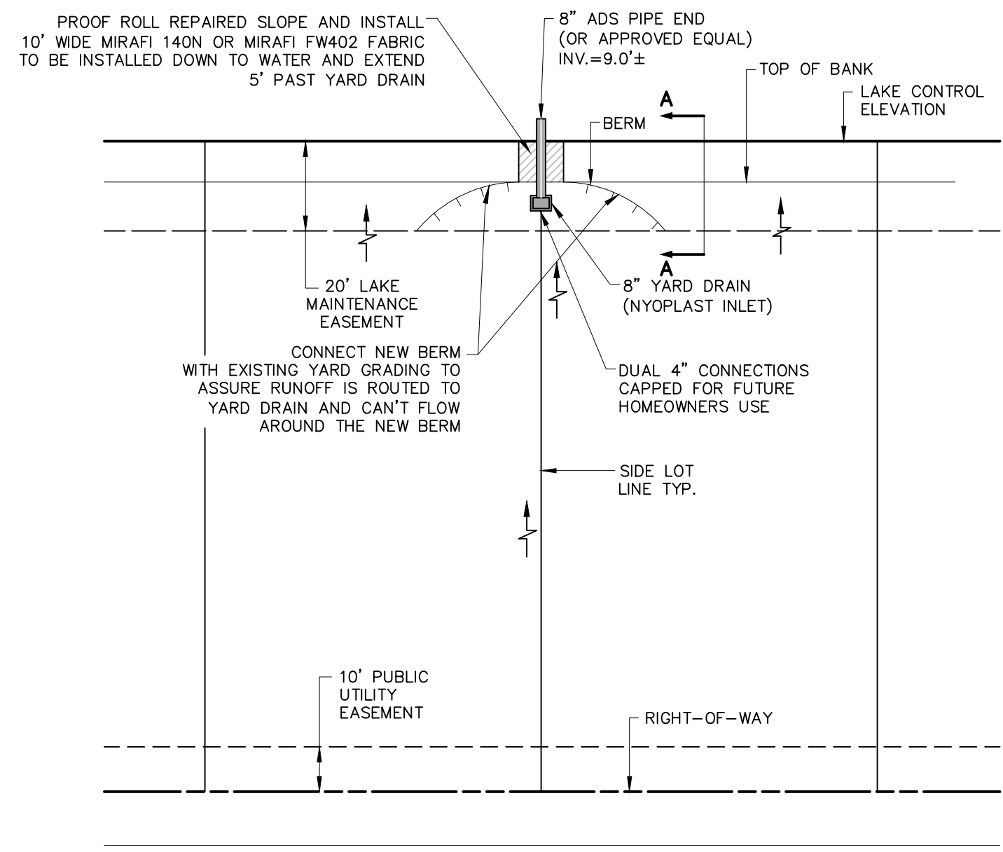
PROPERTY LINE YARD DRAIN INSTALLATION SCALE: 1"=30'
